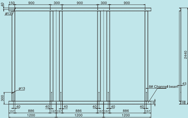
Figure4:Typical basic frame foundation
