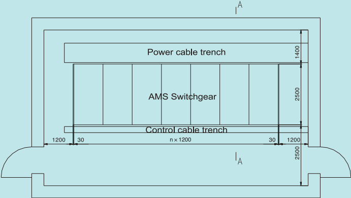
Figure1:plane diagram for switchgear arrangement scheme
