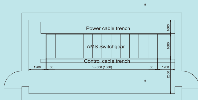
Figure1:plane diagram for switchgear arrangement scheme
