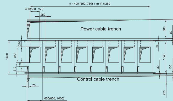
Figure3:Switch-room cable trench arrangement scheme
