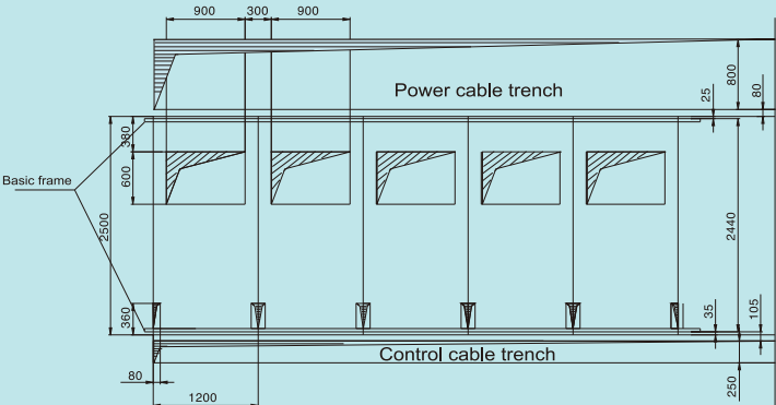
Figure3:Switch-room cable trench arrangement scheme
