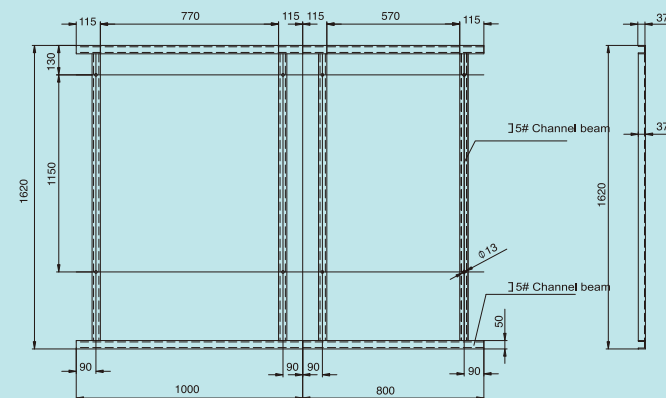
Figure4:Typical basic frame foundation (for 1000mm/800mm width dimension model)
