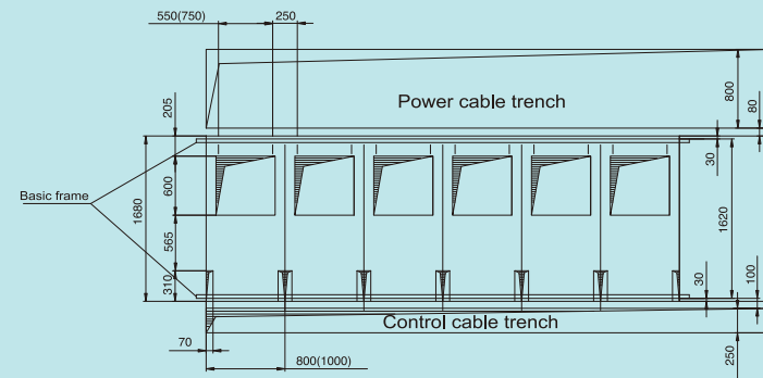
Figure3:Switch-room cable trench arrangement scheme
