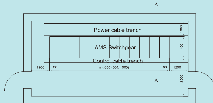
Figure1:plane diagram for switchgear arrangement scheme
